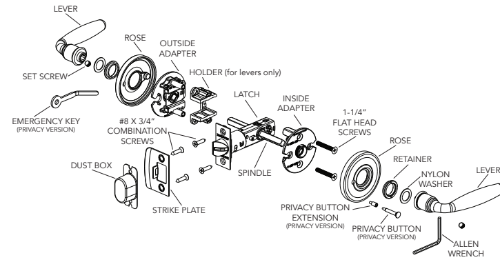
Exploded View (Privacy Function Shown)
